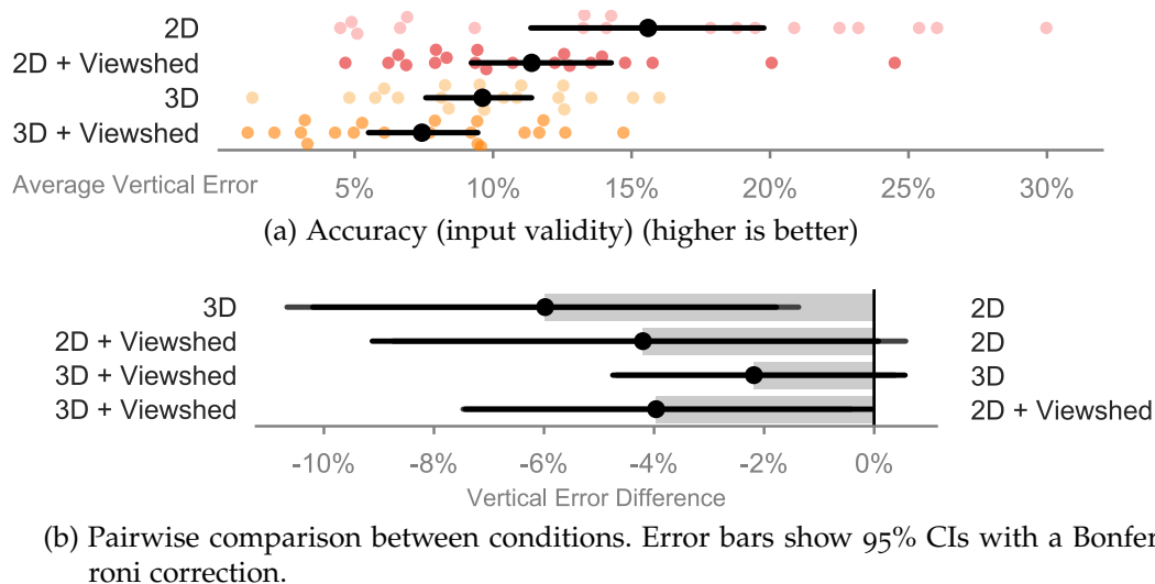
Figure 30: Study results: accuracy (input validity) of lowest visible point trials
