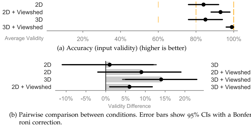
Figure 29: Study results: accuracy (input validity) of lowest-visible-point trials
